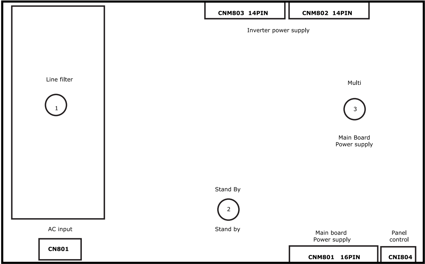
8-4 Power Board Layout
