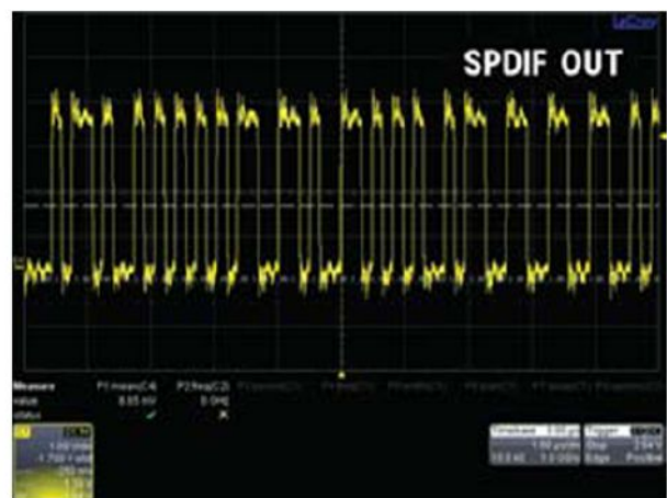
② Monitor OUT , SPDIF OUT
